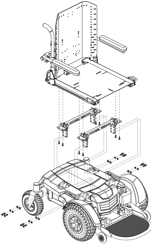
Figure 5. Quantum/Jazzy 1450 Series Power Chair with Synergy Seating System
