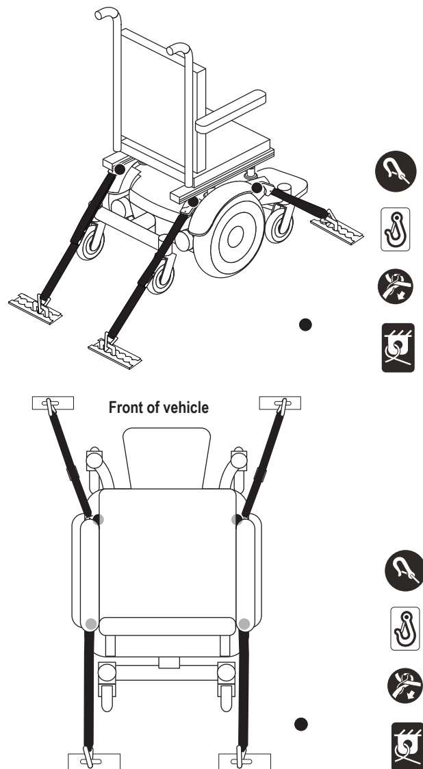
Figure 8. Unoccupied Transit System Securement Points
