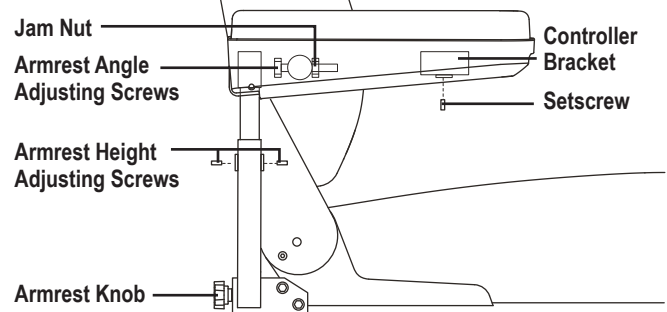
Figure 11. Seatback/Armrest Adjustment
