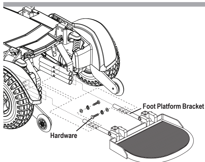
Figure 12. Foot Platform Adjustment
